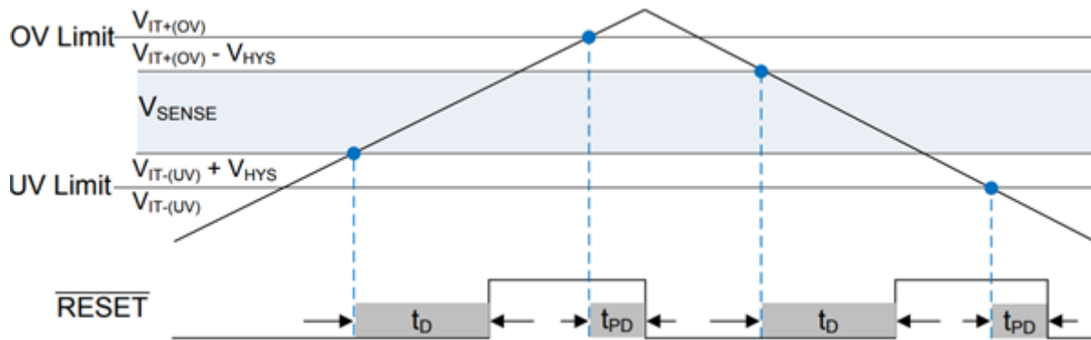
Figure 3. Under-voltage and Over-voltage Window Detector Timing Diagram
