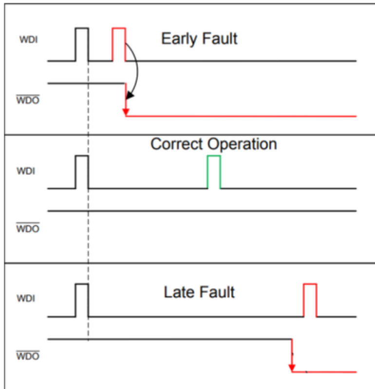
Figure 2. Window Watchdog Timing Diagram
