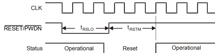
Figure 42. DAC RESET/PWDN
