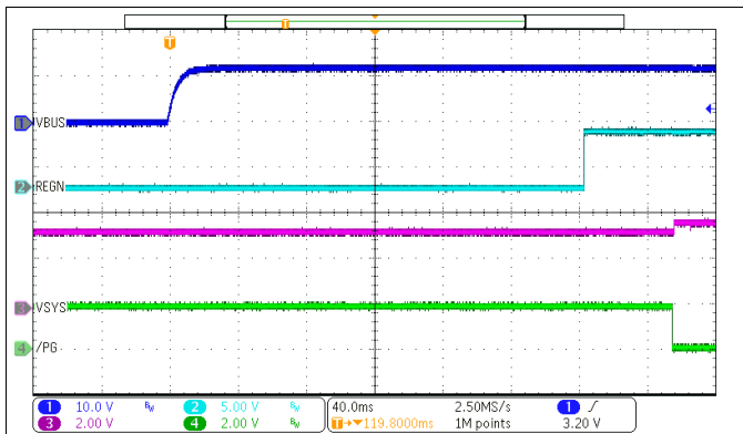
图 47. Power Up with Charge Disabled
