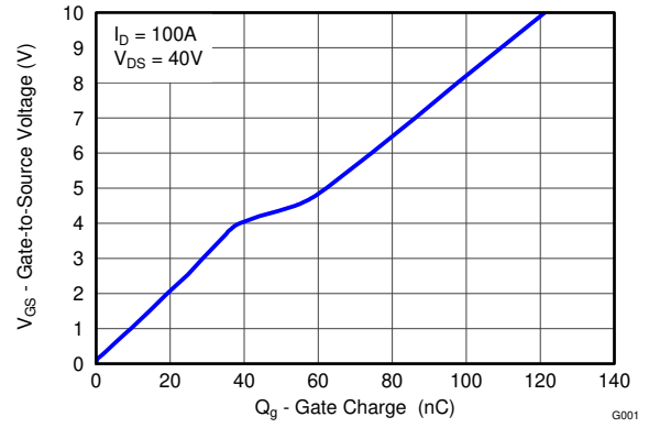
栅极电荷
