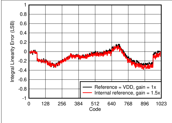
图 7-12. Integral Linearity Error vs Digital Input Code
