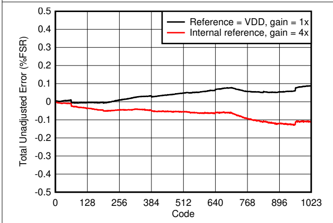
图 7-6. Total Unadjusted Error vs Digital Input Code
