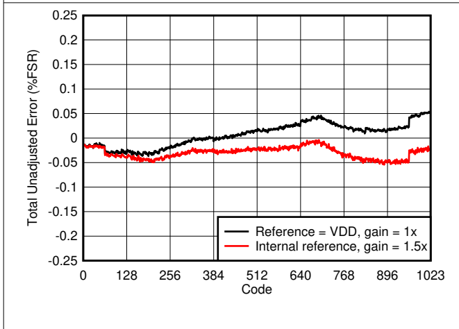
图 7-16. Total Unadjusted Error vs Digital Input Code
