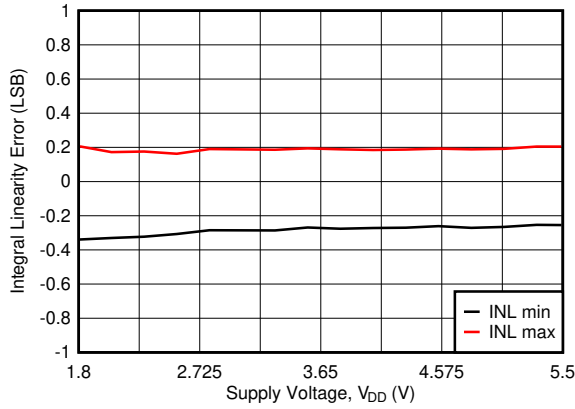
图 7-22. Integral Linearity Error vs Supply Voltage
