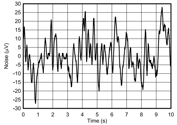
图 7-47. DAC Output Noise: 0.1 Hz to 10 Hz
