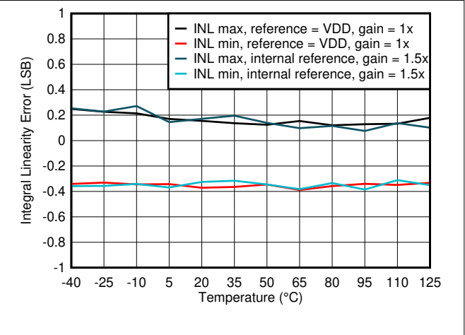
图 7-13. Integral Linearity Error vs Temperature
