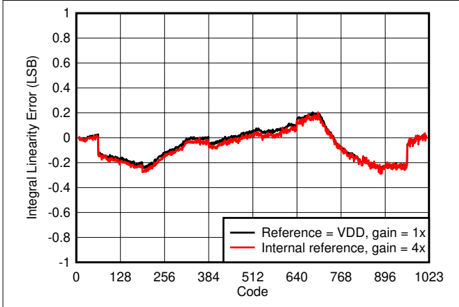
图 7-2. Integral Linearity Error vs Digital Input Code
