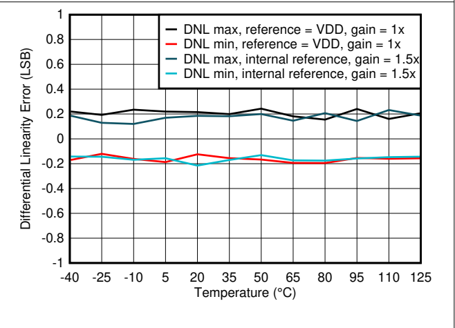
图 7-15. Differential Linearity Error vs Temperature
