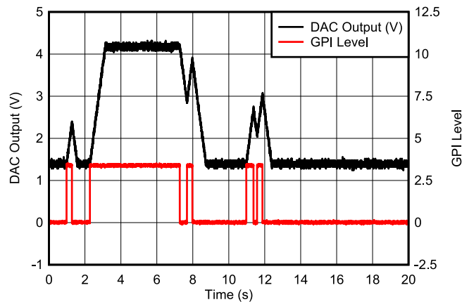
图 9-3. Light Fade-In-Fade-Out With GPI
