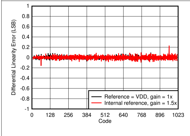
图 7-14. Differential Linearity Error vs Digital Input Code
