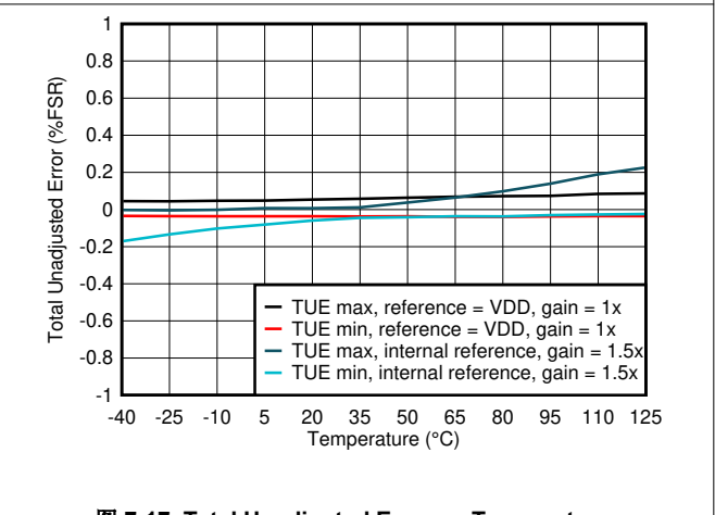
图 7-17. Total Unadjusted Error vs Temperature
