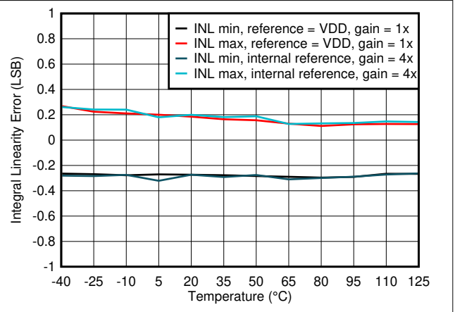
图 7-3. Integral Linearity Error vs Temperature
