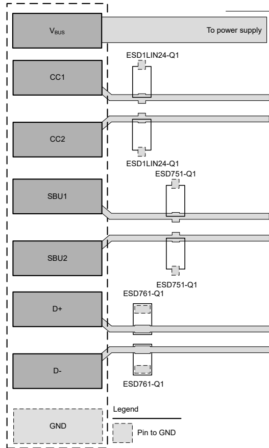
图 10-1. Layout Recommendation
