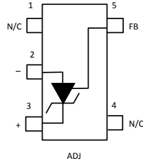
图 4-5. DCK Package 5-Pin SC70 Top View
