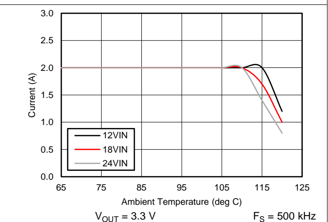
Figure 50. Derating Curve
