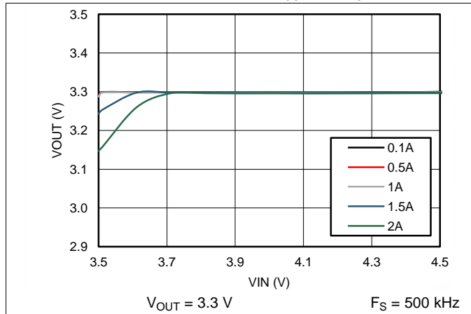
Figure 45. Dropout Voltage
