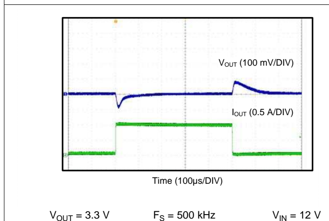
Figure 49. Load Transient
