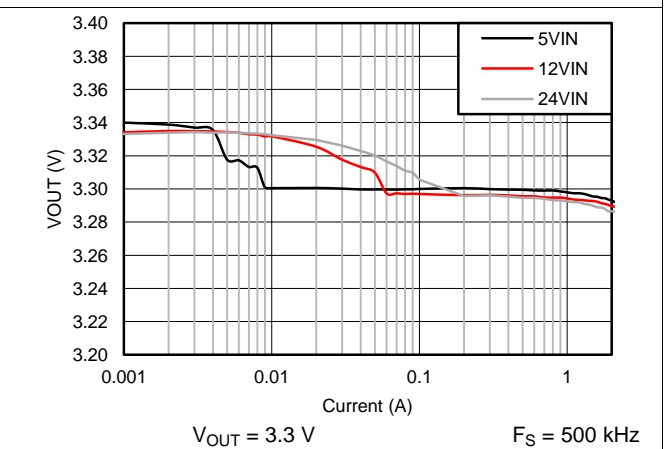
Figure 48. Regulation Curve
