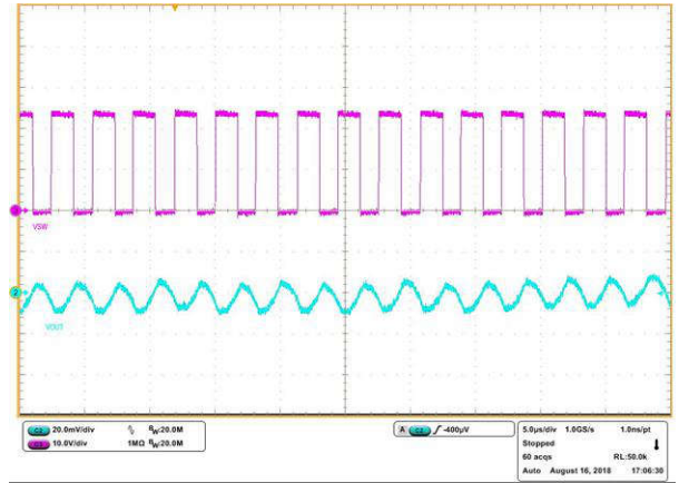
图 7-15. Full-Load Switching
