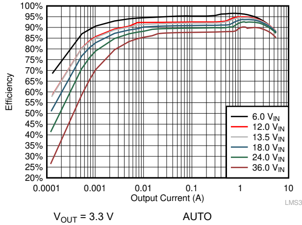
图 9-17. Efficiency
