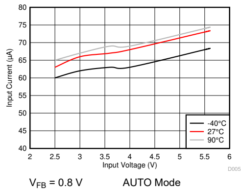
图 6-5. Non-Switching Input Current in AUTO Mode
