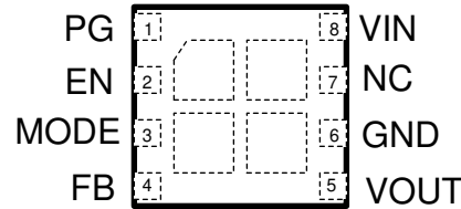
图 5-1. 8-Pins USIP Package (SIL) (Top View)
