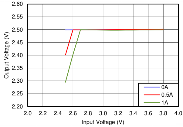
图 7-5. Typical Dropout Behavior, V OUT = 2.5 V
