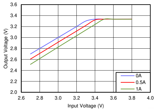
图 7-6. Typical Dropout Behavior, V OUT = 3.3 V
