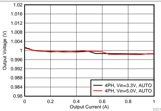
图 50. Output Voltage vs Load Current in PFM/PWM Mode (4-Phase Output)
