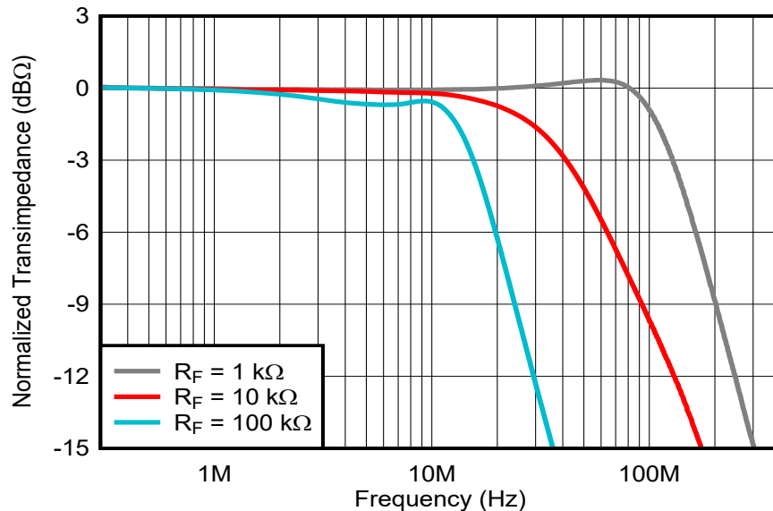
图 9-2. Bandwidth vs Frequency
