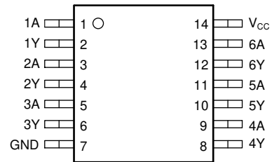
图 5-2. SN74LV6T06-Q1 PW Package, 14-Pin TSSOP (Top View)
