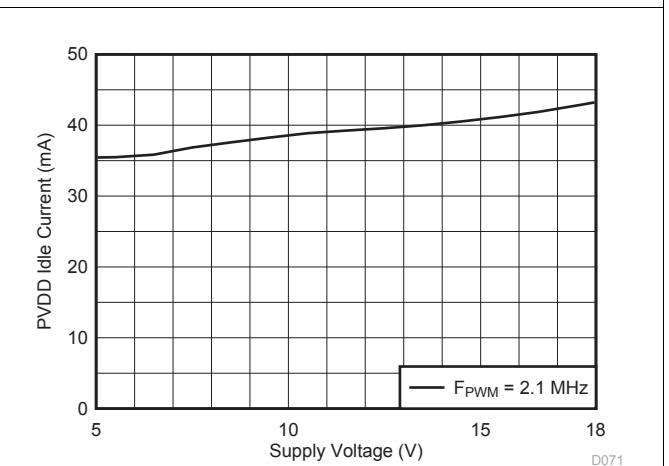
图 16. PVDD Idle Current vs Voltage
