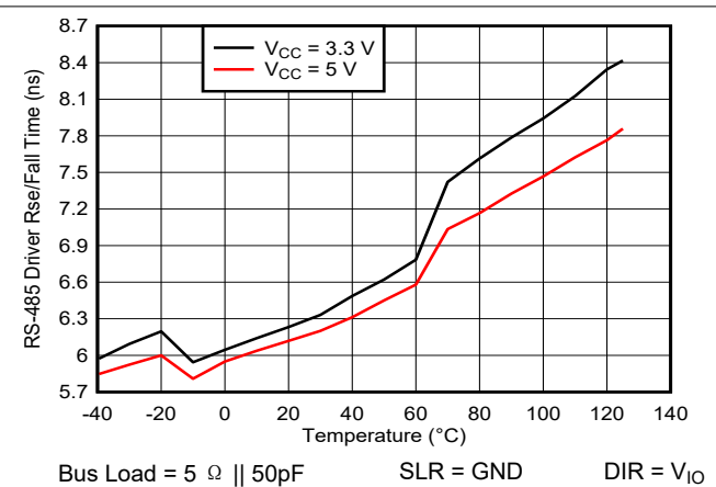
图 5-10. RS-485 20Mbps Driver Rise or Fall Time vs Temperature
