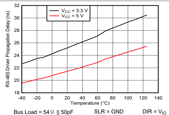
图 5-12. RS-485 20Mbps Driver Propagation Delay vs Temperature
