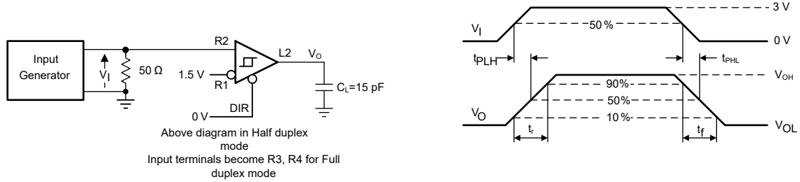
图 6-6. Measurement of RS-485 Receiver Output Rise and Fall Times and Propagation Delays
