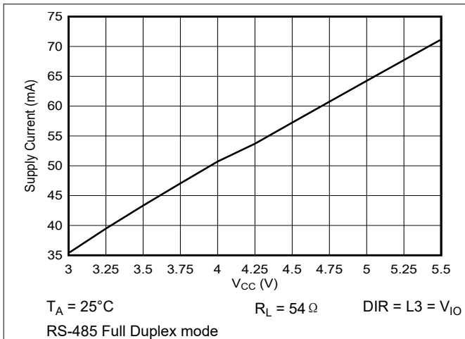
图 5-7. RS-485 Supply Current vs Supply Voltage
