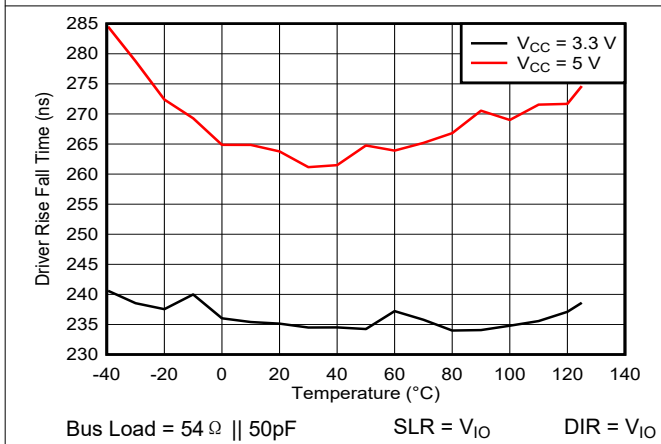
图 5-9. RS-485 500kbps Driver Rise or Fall Time vs Temperature
