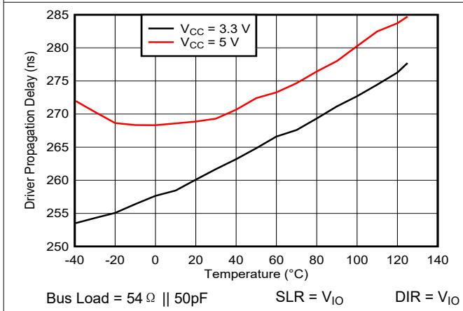
图 5-11. RS-485 500kbps Driver Propagation Delay vs Temperature
