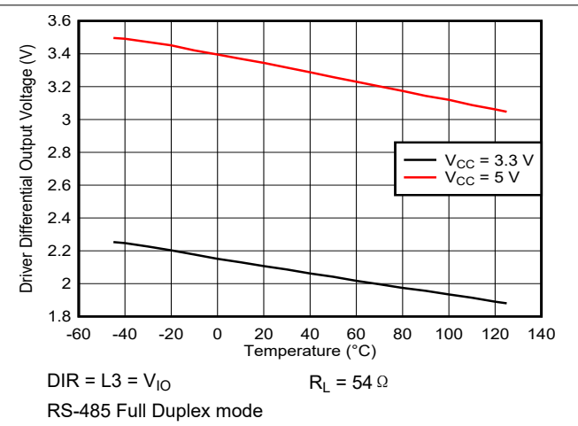
图 5-8. RS-485 Driver Differential Output Voltage vs Temperature
