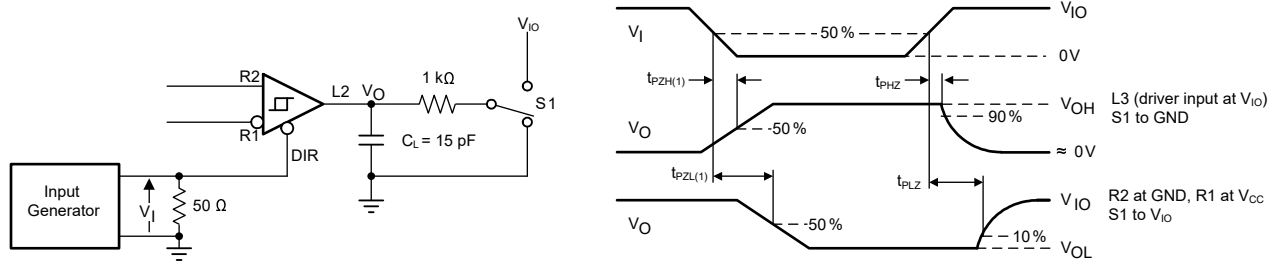
图 6-7. Measurement of RS-485 Receiver Enable and Disable Times in Half Duplex Mode
