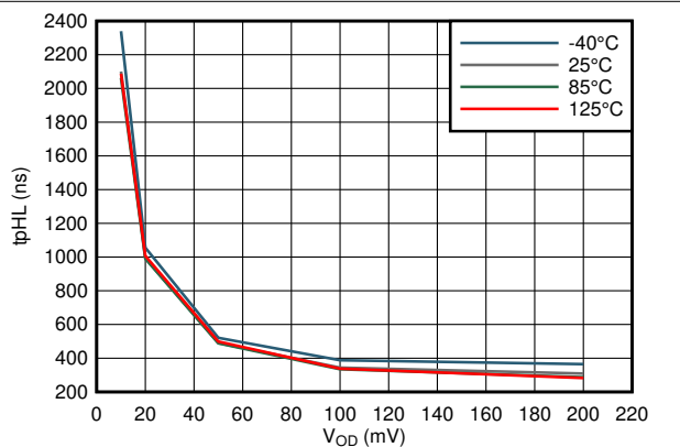
图 7-29. Propagation Delay High-Low vs Input Overdrive
