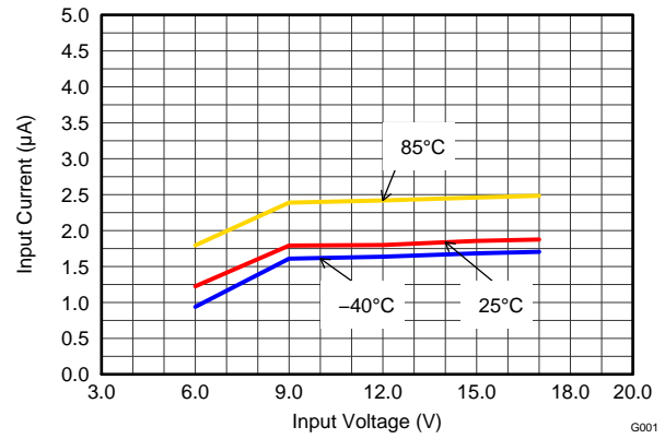
Figure 2. Shutdown Current
