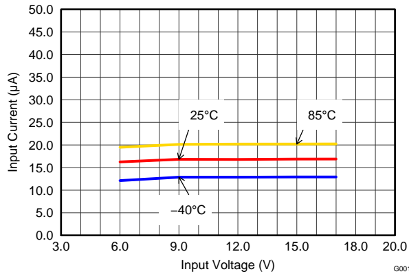
Figure 1. Quiescent Current
