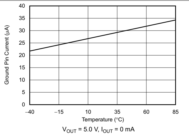
图 6-22. Ground Pin Current vs Temperature
