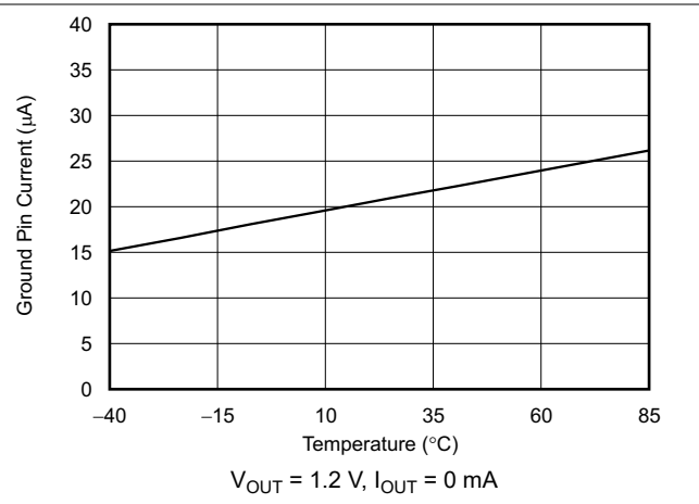
图 6-20. Ground Pin Current vs Temperature
