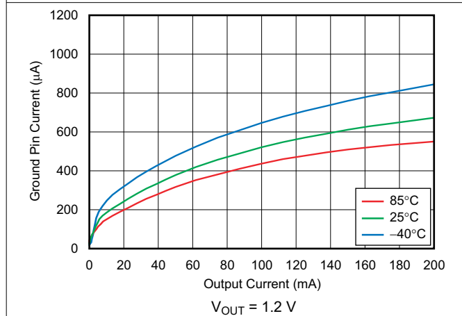
图 6-23. Ground Pin Current vs Output Current
