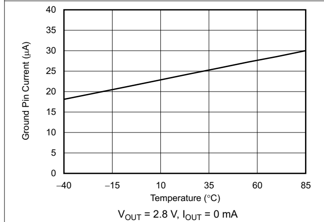
图 6-21. Ground Pin Current vs Temperature
