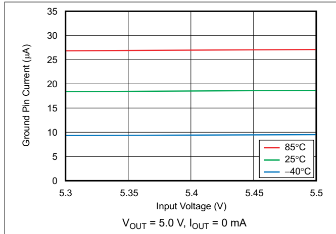
图 6-19. Ground Pin Current vs Input Voltage
