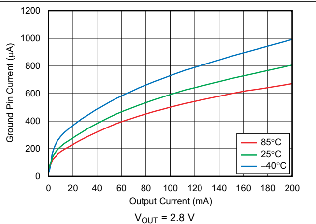
图 6-24. Ground Pin Current vs Output Current
