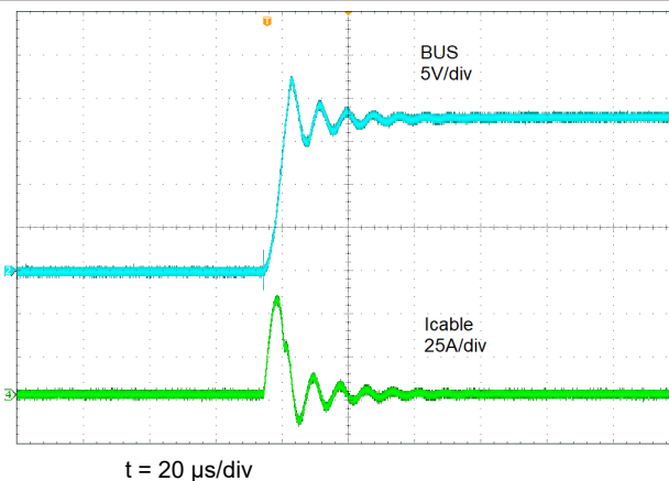
图 9-6. DC-DC VIN Floating, BUS Shorted to Battery
