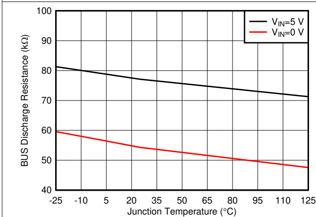
图 6-3. BUS Discharge Resistance (OVP) vs Temperature
