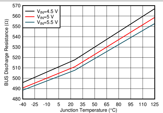
图 6-4. BUS Discharge Resistance (Mode Change) vs Temperature
