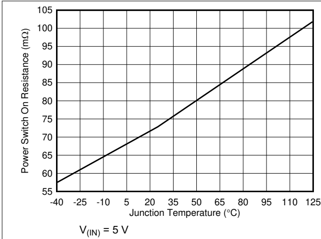
图 6-1. Power Switch On-Resistance vs Temperature
