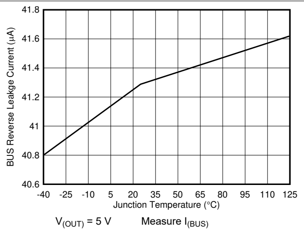
图 6-2. Reverse Leakage Current vs Temperature
