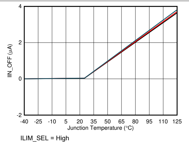
图 6-6. Disabled IN Supply Current vs Temperature
