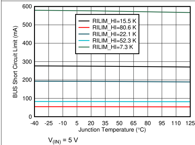
图 6-5. VBUS Short-Circuit Current Limit vs Temperature
