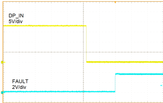
图 6-24. DP_IN Short-to-Battery Recovery
