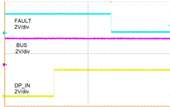
图 6-25. DP_IN Short-to- V_{\text{BUS}}
