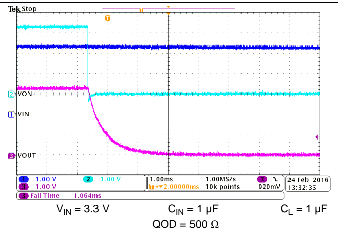
Figure 25. Fall Time ( t_F ) at V_{IN} = 3.3 V
