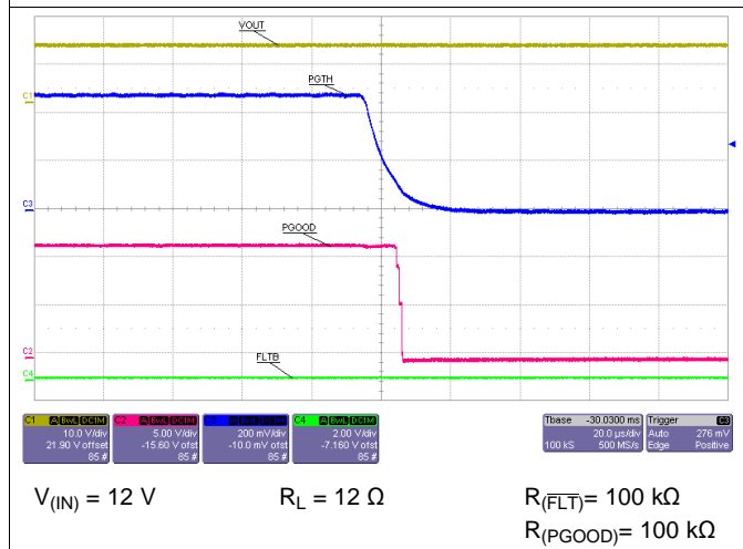
Figure 39. Power Good Delay (Falling)
