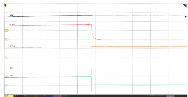
OV threshold set to 16.7\text{ V} , V_{IN} ramped up from 12\text{ V} to 17\text{ V}
