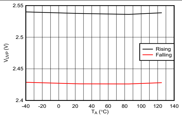
图 7-6. IN Undervoltage Threshold vs Temperature
