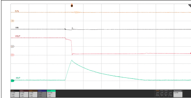
V_{IN} = 12\text{ V} , R_{ILM} = 715\text{ }\Omega , I_{OUT} stepped from Open \rightarrow Short-circuit to GND
