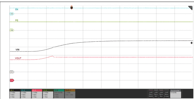
ROVCSSEL = Open, C OUT = 220 μF, I OUT = 200 mA, V IN ramped up from 5 V to 7.5 V
