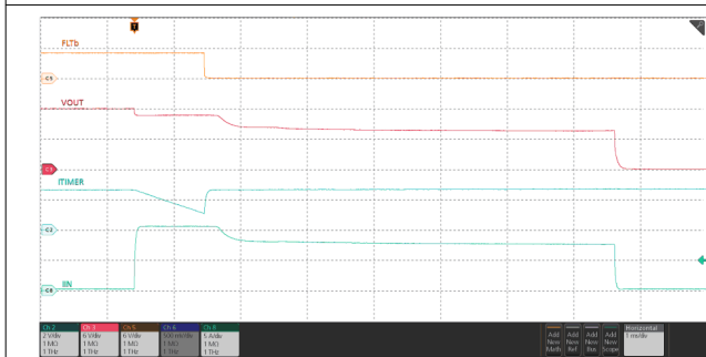
V IN = 12 V, C TIMER = 1.3 nF, C OUT = 220 μF, R ILM = 715 Ω, I OUT stepped from 0 A → 11 A
