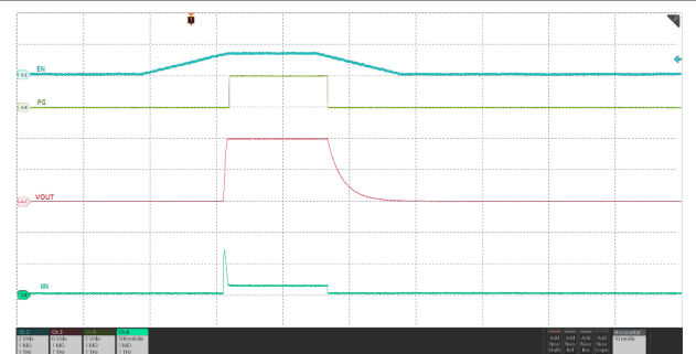
图 7-28. Time to Thermal Shut-Down During Inrush State
