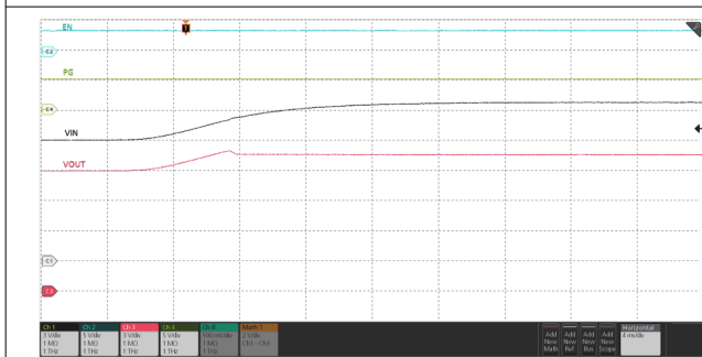
ROVCSSEL = 390 kΩ, C OUT = 220 μF, I OUT = 200 mA, V IN ramped up from 12 V to 16.5 V
