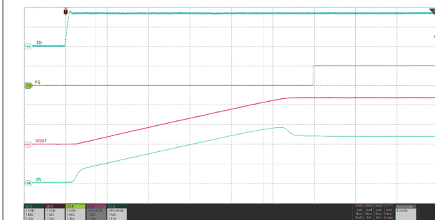
V_{IN} = 12\text{ V} , C_{OUT} = 470\ \mu\text{F} , R_{OUT} = 10\ \Omega , C_{dVdt} = 5100\text{ pF} , V_{EN/UVLO} stepped up to 3.3\text{ V}
