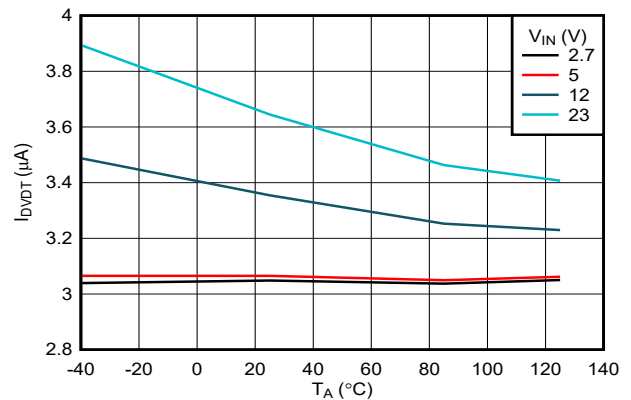
图 7-24. DVDT Charging Current vs Temperature
