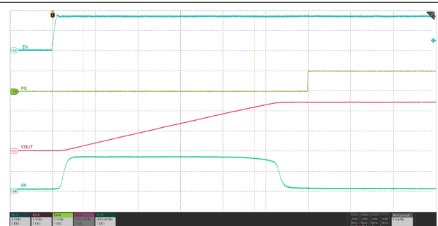
V_{IN} = 12\text{ V} , C_{OUT} = 470\ \mu\text{F} , C_{dVdt} = 5100\text{ pF} , V_{EN/UVLO} stepped up to 3.3\text{ V}
