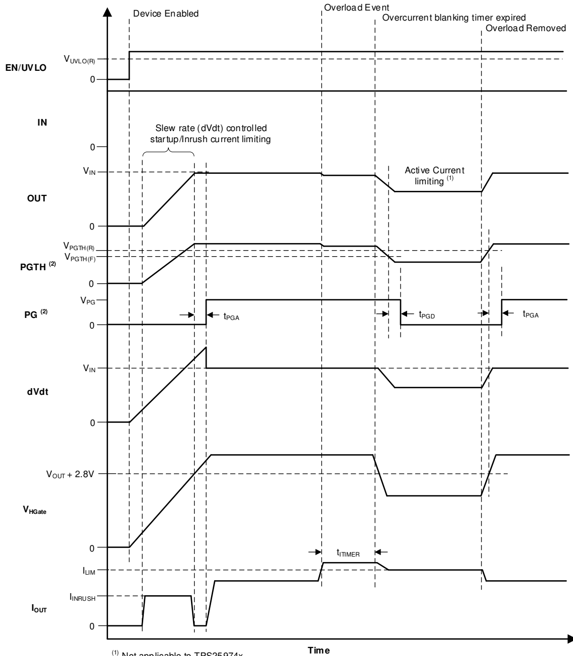
图 8-13. TPS25972x, TPS25974x PG Timing Diagram
