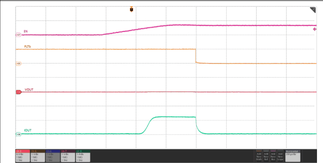
V_{IN} = 12\text{ V} , C_{OUT} = \text{Open} , I_{OUT} short-circuit to GND, R_{ILM} = 715\text{ }\Omega , V_{EN/UVLO} stepped from 0\text{ V} \rightarrow 3.3\text{ V}
