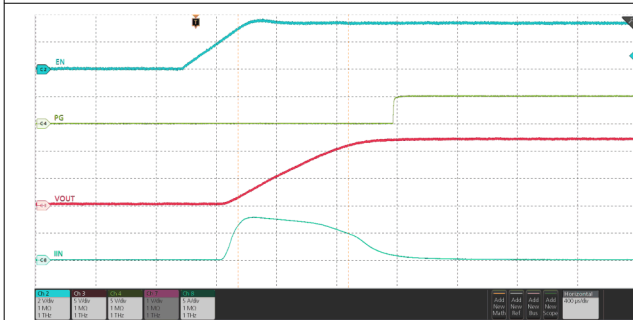
V_{IN} = 12\text{ V} , C_{OUT} = 470\ \mu\text{F} , C_{dVdt} = \text{Open} , V_{EN/UVLO} stepped up to 3.3\text{ V}
