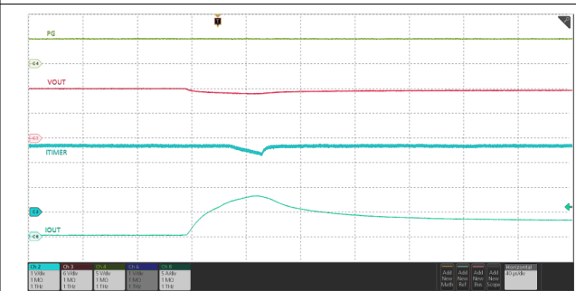
V IN = 12 V, C TIMER = 120 pF, C OUT = 470 μF, R ILM = 715 Ω, I OUT ramped from 0 A → 8 A → 4 A within 100 μs
