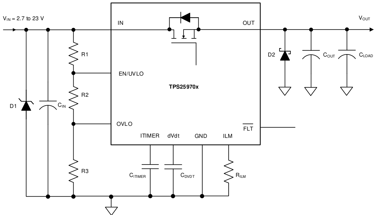
图 9-10. Circuit Implementation With Optional Protection Components
