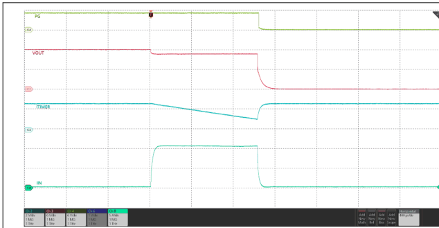
V_{IN} = 12\text{ V} , C_{TIMER} = 1.3\text{ nF} , C_{OUT} = 470\text{ }\mu\text{F} , R_{ILM} = 715\text{ }\Omega , I_{OUT} stepped from 0\text{ A} \rightarrow 11\text{ A}
