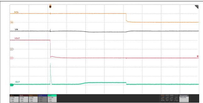
V_{IN} = 12\text{ V} , R_{ILM} = 715\text{ }\Omega , I_{OUT} stepped from Open \rightarrow Short-circuit to GND
