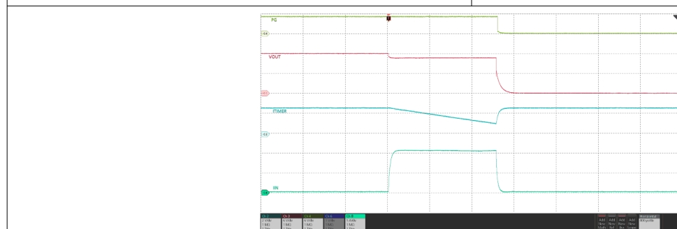
图 9-6. Circuit Breaker Response
