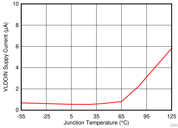
图 7-4. VLDOIN Supply Current vs Junction Temperature
