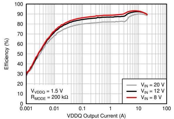
图 7-21. Efficiency
