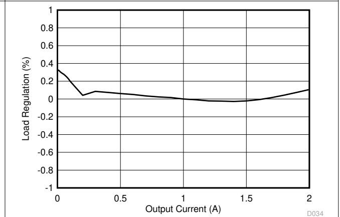
图 8-5. Tps562200 Load Regulation, V_I = 12V
