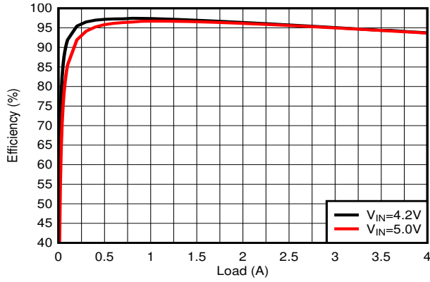
图 8-21. PWM Efficiency
