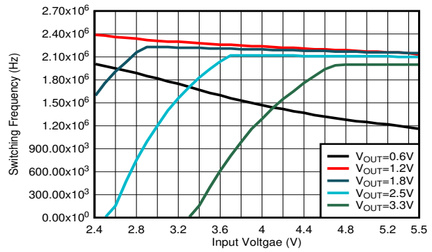
图 8-24. Switching Frequency
