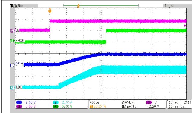
Load = 0.6 \Omega TPS62826
