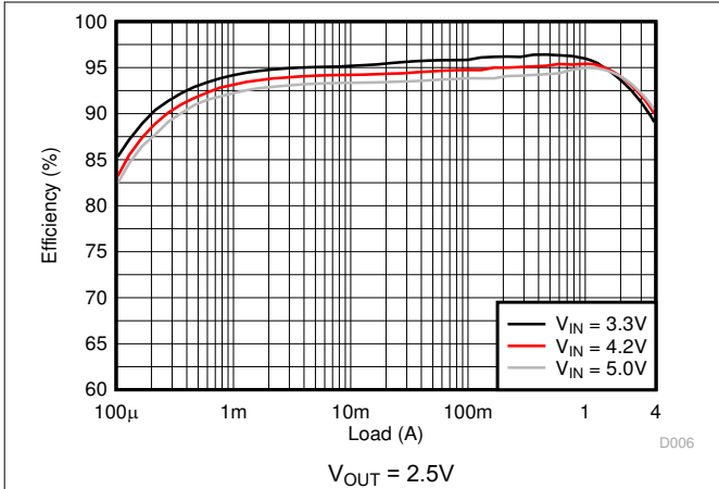
图 8-15. Efficiency
