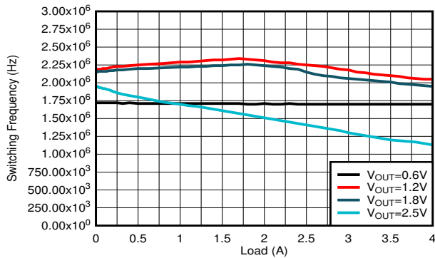
图 8-23. Switching Frequency
