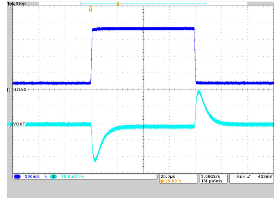
图 9-27. Load Transient Response
