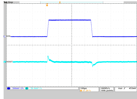
图 9-33. Line Transient Response
