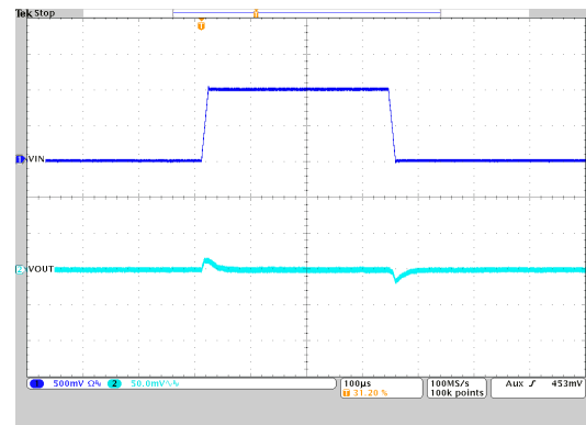
图 9-35. Line Transient Response
