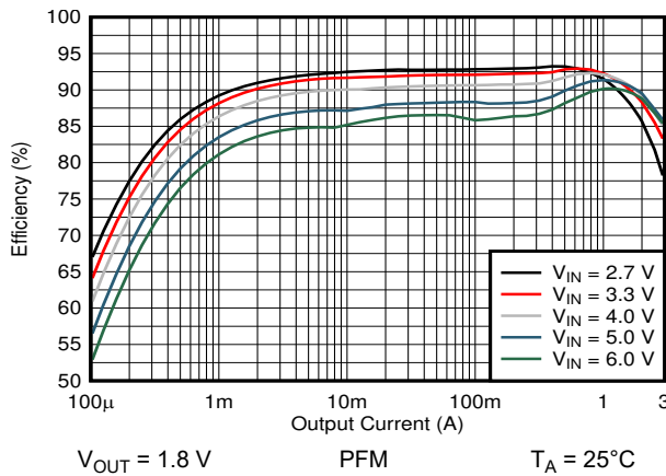
图 10-4. Efficiency Versus Output Current
