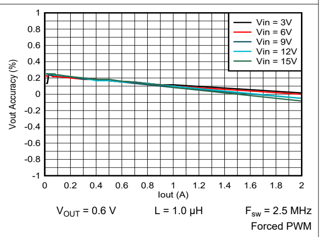
图 9-32. Output Voltage vs Output Current
