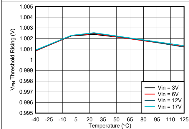
图 7-17. Precision Enable Threshold vs Temperature
