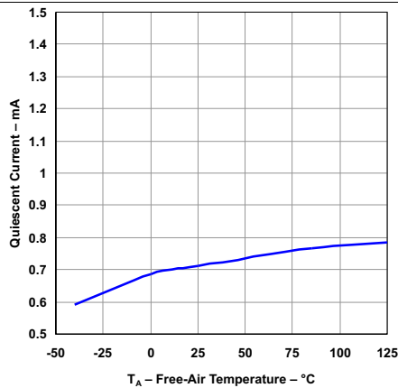
V_{IN} = 6\text{ V} I_{OUT} = 0\text{ A} V_{EN} = V_{IN} TPS73801
