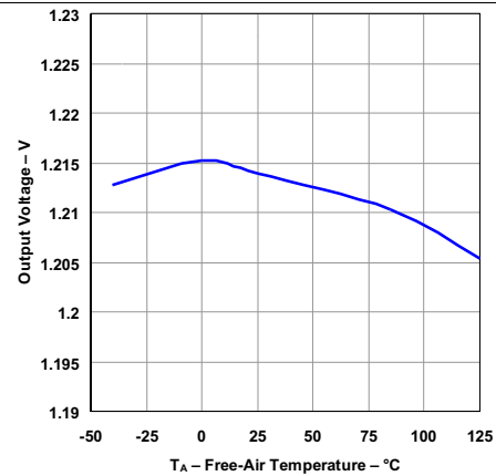
V_{IN} = 6\text{ V} I_{OUT} = 1\text{ mA} TPS73801
