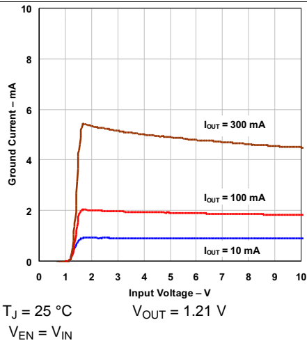
Figure 7. Ground Current vs Input Voltage
