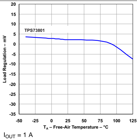
Figure 19. Load Regulation vs Temperature
