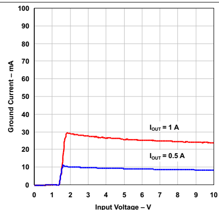
T_J = 25\text{ °C} V_{OUT} = 1.21\text{ V} V_{EN} = V_{IN} TPS73801
