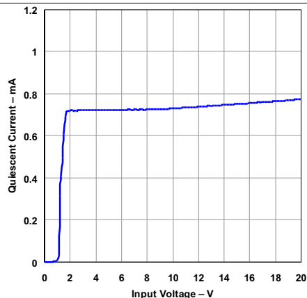
T_J = 25\text{ °C} R_{OUT} = 4.3\text{ k}\Omega V_{EN} = V_{IN} TPS73801
