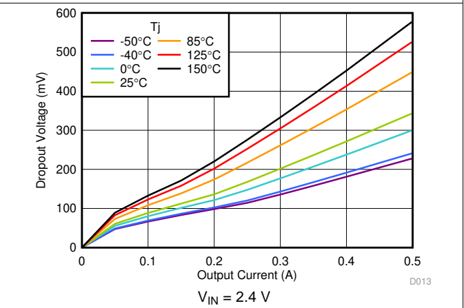
图 6. Dropout Voltage vs I_{OUT}
