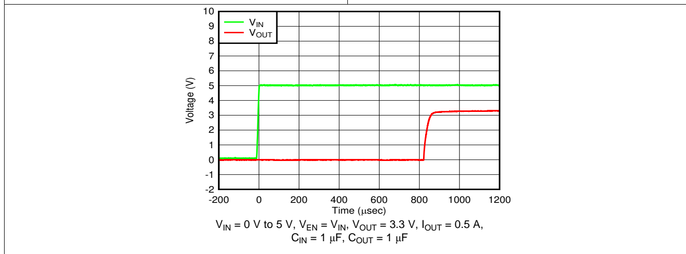
图 33. Start-Up With Enable Pin Tied to Input
