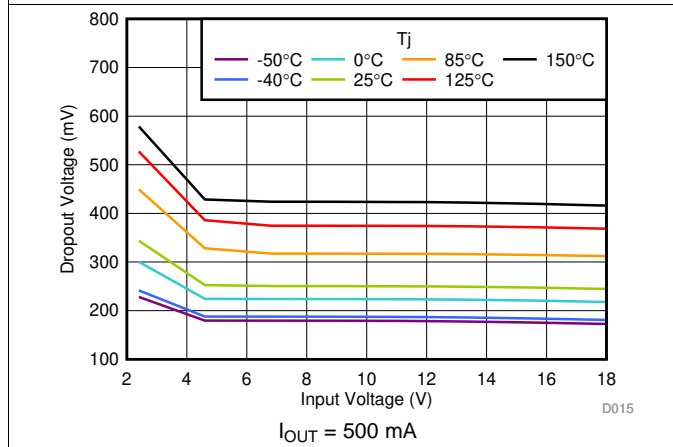
图 5. Dropout Voltage vs V_{IN}
