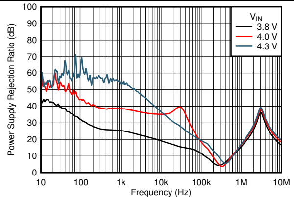
图 20. PSRR vs Frequency and V_{IN}
