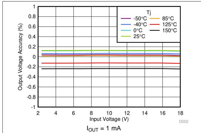
图 1. Line Regulation vs V_{IN}
