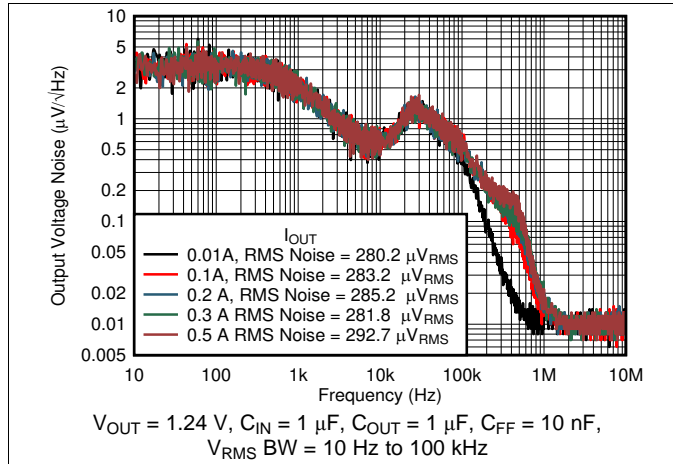
图 25. Output Noise ( V_n ) vs Frequency and I_{OUT}
