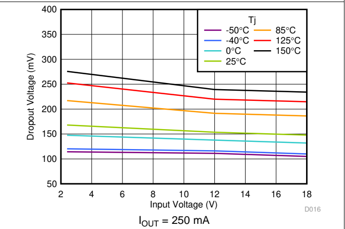
图 4. Dropout Voltage vs V_{IN}
