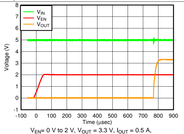
图 32. Start-Up With Enable
