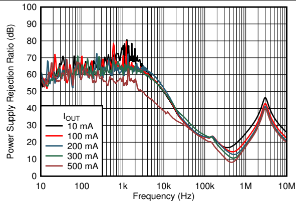
图 19. PSRR vs Frequency and I_{OUT}
