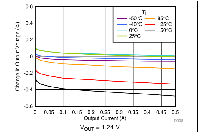
图 2. Load Regulation vs I_{OUT}
