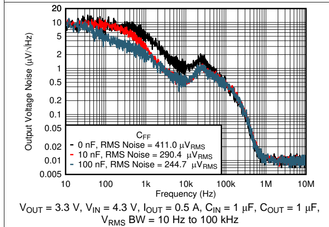
图 27. Output Noise ( V_n ) vs Frequency and C_{FF}
