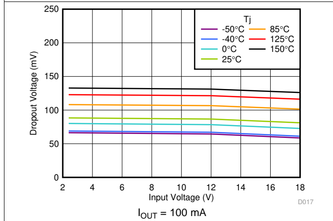
图 3. Dropout Voltage vs V_{IN}
