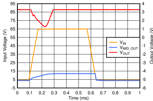
V_{IN} = 4\text{ V to } 65\text{ V} , V_{IN} ramp rate = 1\text{ V}/\mu\text{ s} , V_{OUT} = 3.3\text{ V} , I_{OUT} = 50\text{ mA}
