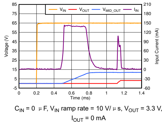
图 6-12. Fast Start-Up (Inrush Current)
