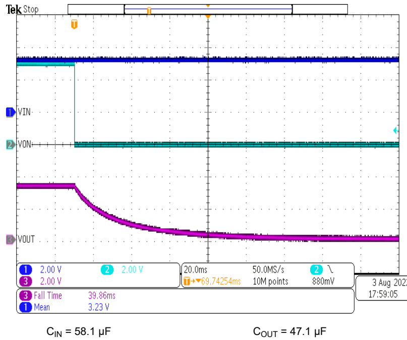
图 9-2. Fall Time ( R_{QOD} = 1 k\Omega )
