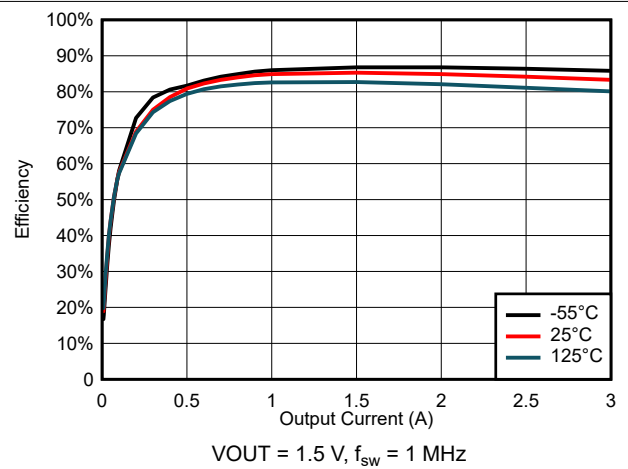
图 6-42. Efficiency for V_{\text{IN}} = 5\text{ V}
