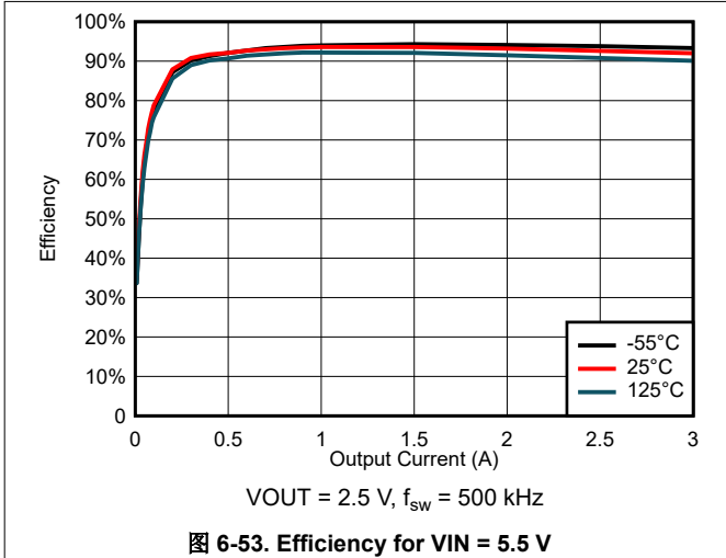
图 6-53. Efficiency for V_{\text{IN}} = 5.5\text{ V}
