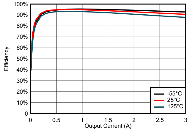
图 6-30. Efficiency for V_{\text{IN}} = 3.3\text{ V}
