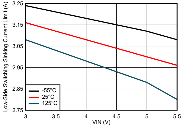
图 6-13. Low-Side Switch Sinking Current Limit Variation
