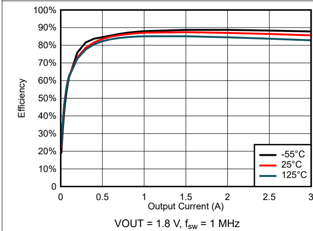
图 6-43. Efficiency for V_{\text{IN}} = 5\text{ V}
