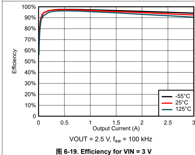
图 6-19. Efficiency for V_{IN} = 3\text{ V}
