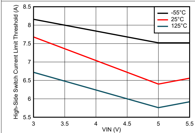
图 6-11. High-Side Switch Current Limit Threshold Variation
