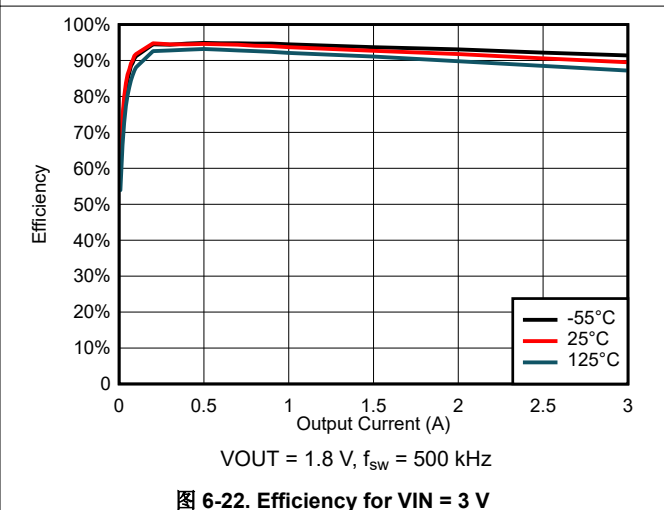
图 6-22. Efficiency for V_{IN} = 3\text{ V}
