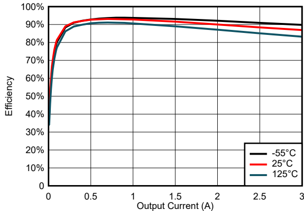
图 6-29. Efficiency for V_{\text{IN}} = 3.3\text{ V}
