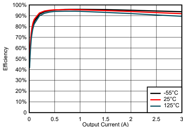
图 6-31. Efficiency for V_{\text{IN}} = 5\text{ V}
