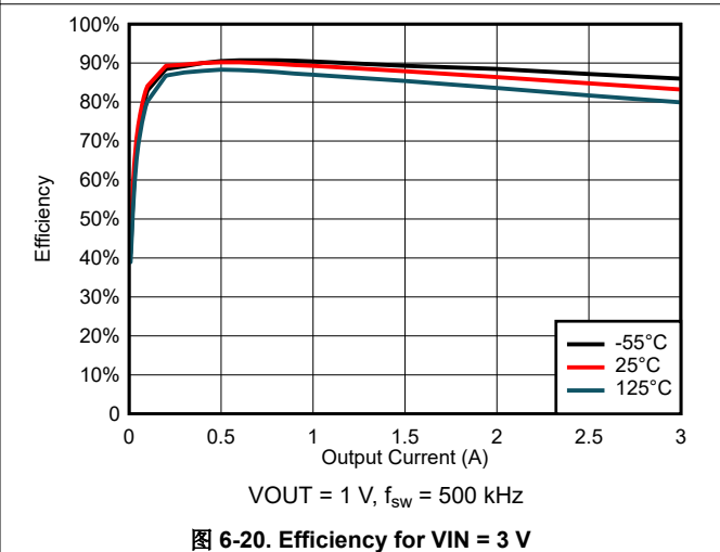
图 6-20. Efficiency for V_{IN} = 3\text{ V}
