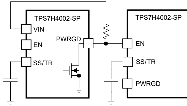
图 7-5. Sequential Start-Up Sequence
