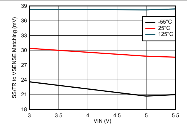
图 6-10. SS/TR to VSENSE Matching Variation
