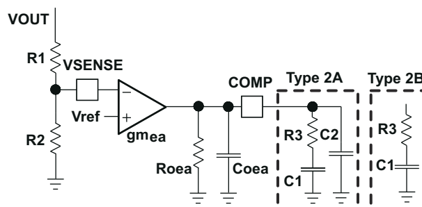
图 7-8. Types of Frequency Compensation
