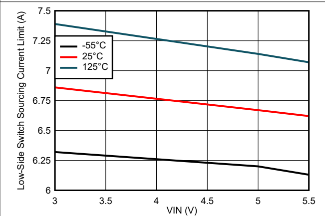
图 6-12. Low-Side Switch Sourcing Current Limit Variation
