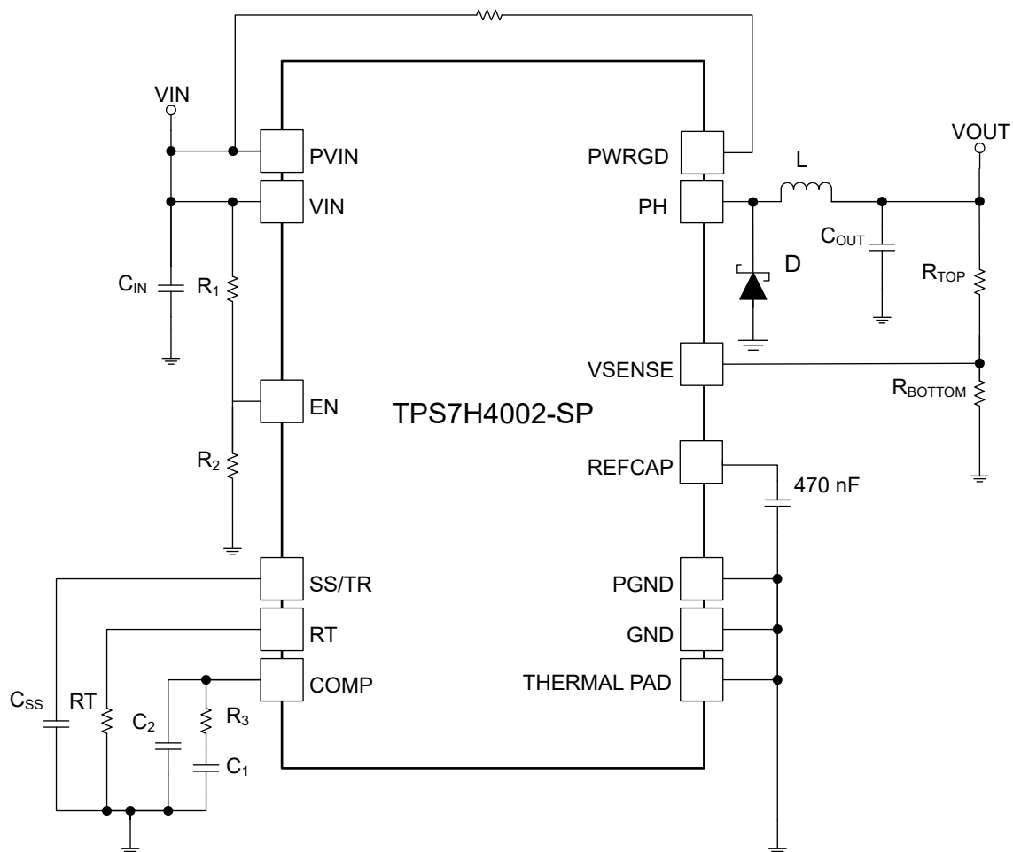
图 8-1. Typical Application Schematic
