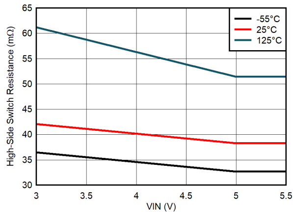
图 6-15. High-Side Switch Resistance Variation
