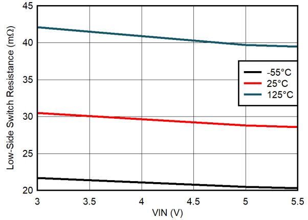
图 6-14. Low-Side Switch Resistance Variation
