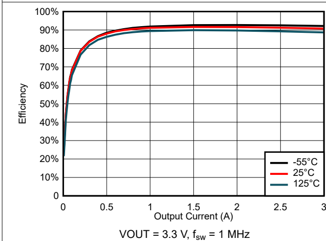
图 6-45. Efficiency for V_{\text{IN}} = 5\text{ V}
