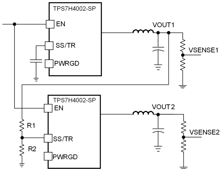
图 7-7. Ratiometric and Simultaneous Start-Up Sequence
