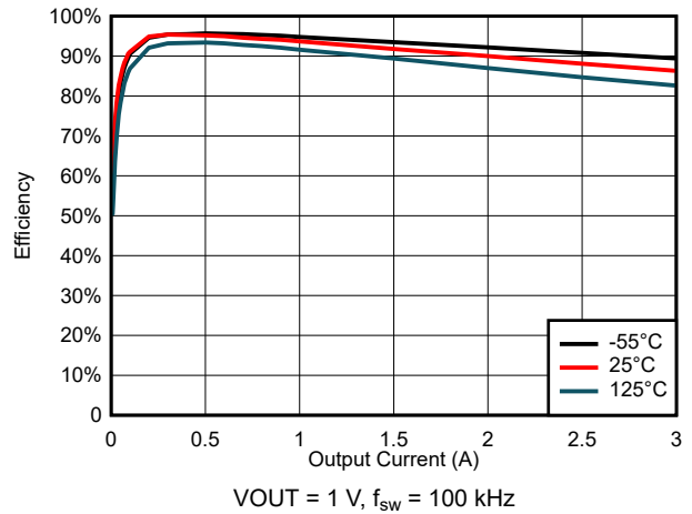
图 6-16. Efficiency for VIN = 3 V
