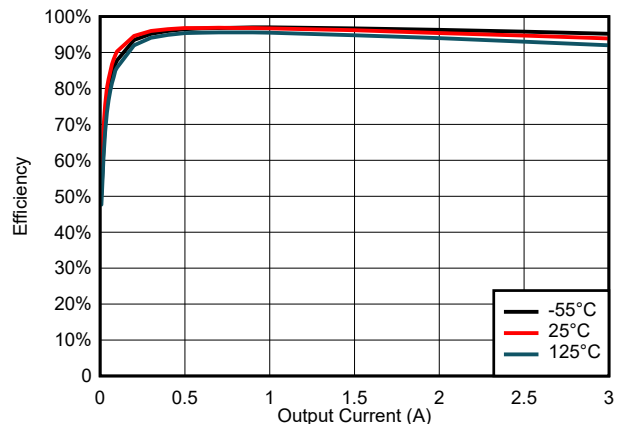
图 6-32. Efficiency for V_{\text{IN}} = 5\text{ V}
