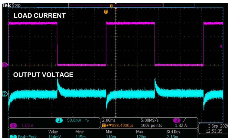
图 8-3. 3-A Step Response for 500-kHz Switching Operation
