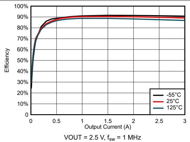
图 6-44. Efficiency for V_{\text{IN}} = 5\text{ V}
