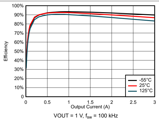
图 6-46. Efficiency for V_{\text{IN}} = 5.5\text{ V}
