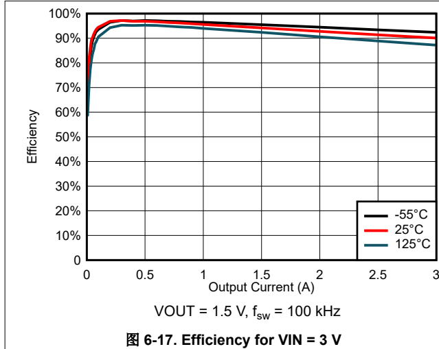
图 6-17. Efficiency for V_{IN} = 3\text{ V}
