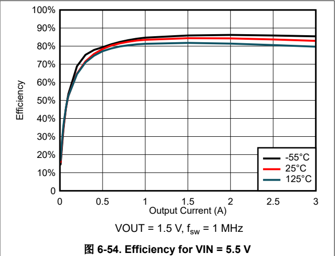
图 6-54. Efficiency for V_{\text{IN}} = 5.5\text{ V}
