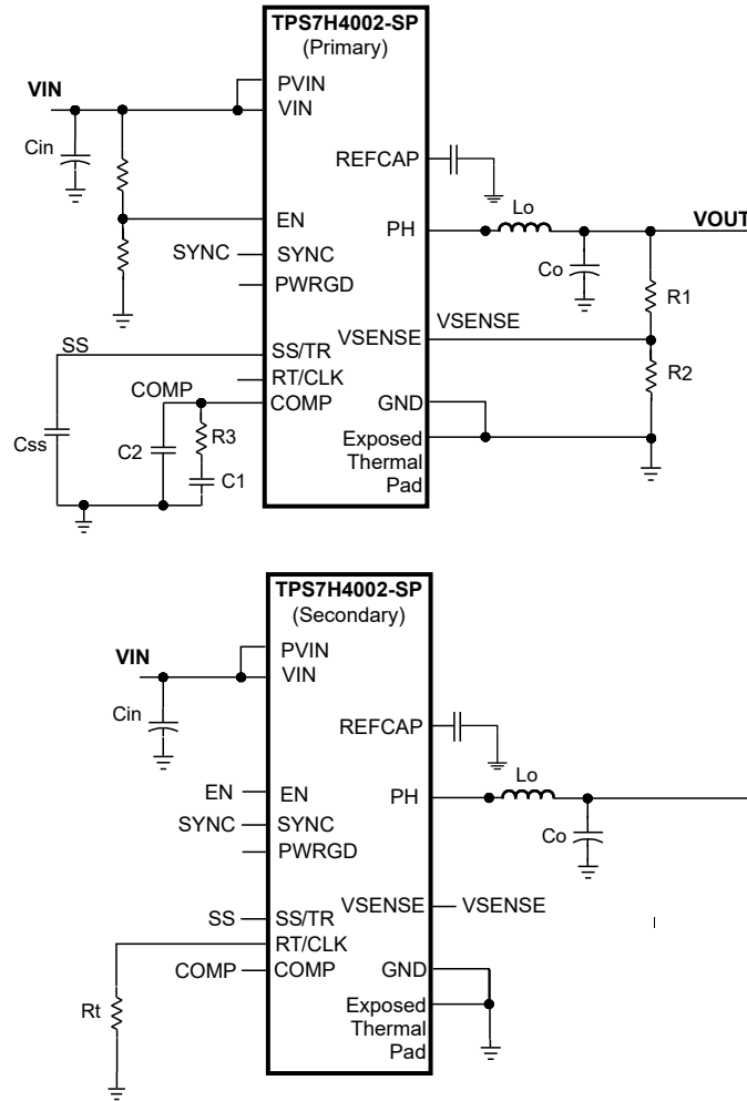
图 8-2. Parallel Configuration Showing Primary and Secondary
