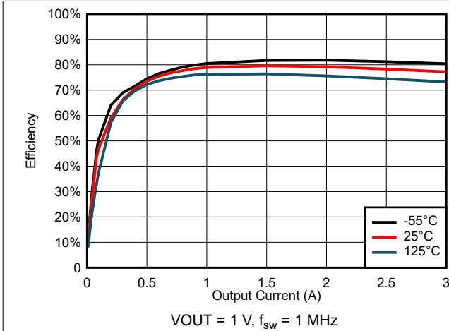
图 6-41. Efficiency for V_{\text{IN}} = 5\text{ V}
