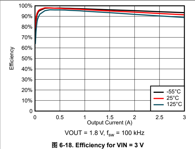
图 6-18. Efficiency for V_{IN} = 3\text{ V}
