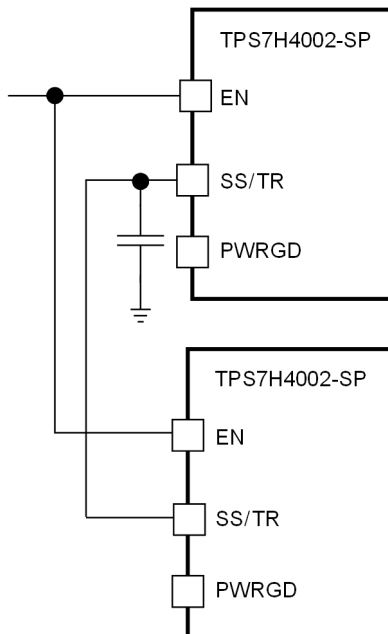
图 7-6. Ratiometric Start-Up Sequence
