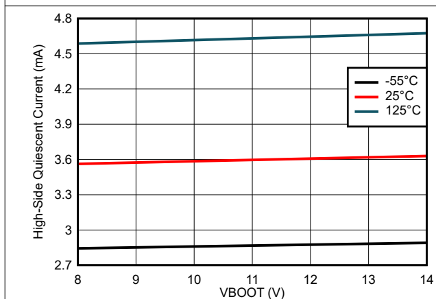
图 7-41. High-Side Quiescent Current vs BOOT Voltage
