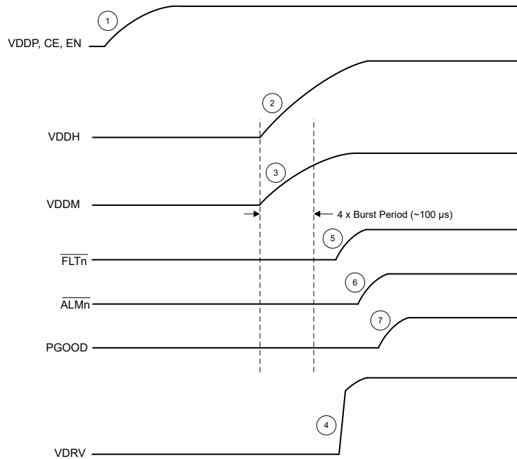
图 8-11. TPSI310x-Q1 典型启动 ( CE = EN = VDDP , FLTn_CMP = 0 , ALMn_CMP = 0 )
