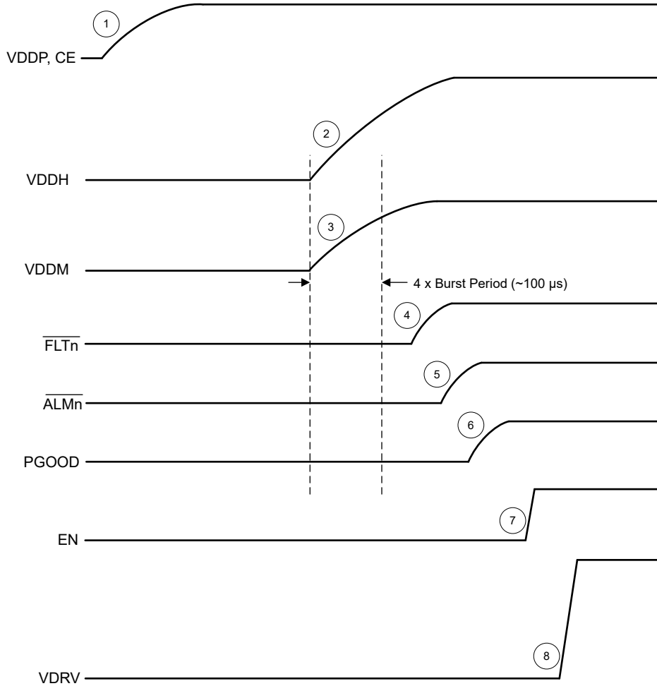
图 8-10. TPSI310x-Q1 典型启动 ( CE = VDDP , FLTn_CMP = 0 , ALMn_CMP = 0 )
