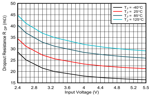
图 6-5. Dropout Resistance R DP
