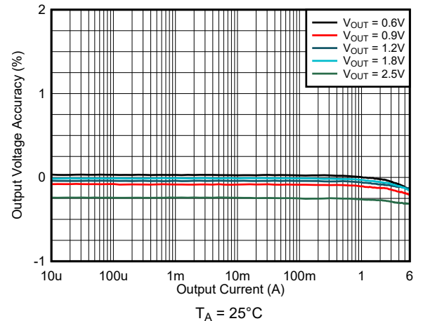
图 8-23. Load Regulation V_{IN} = 3.3\text{ V} and FPWM
