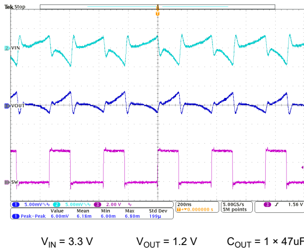
图 8-28. FPWM Operation I_{OUT} = 3\text{ A}
