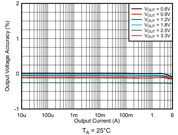
图 8-21. Load Regulation V_{IN} = 5.0\text{ V} and FPWM
