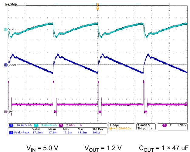
图 8-29. PSM Operation I_{OUT} = 0.1\text{ A}
