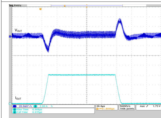
图 8-30. FPWM Operation I_{OUT} = 3\text{ A}
