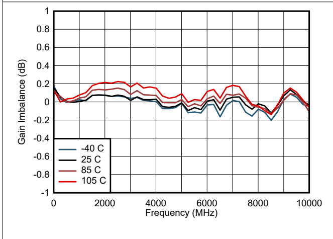
图 6-69. Gain Imbalance
