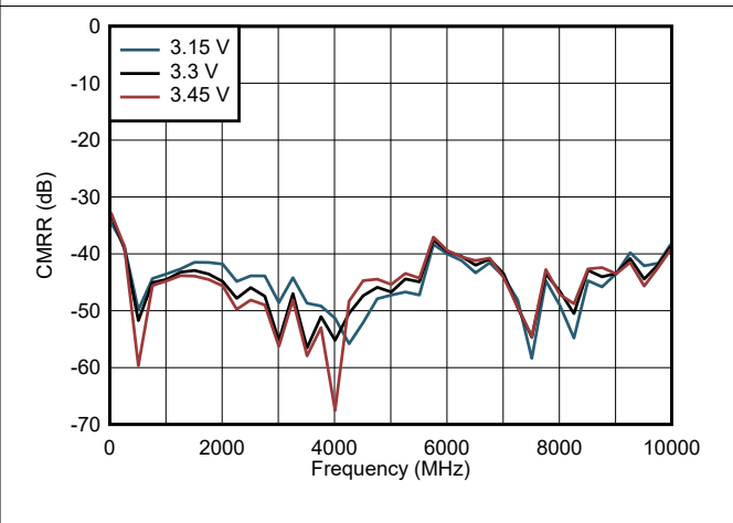
图 6-72. CMRR Across VDD
