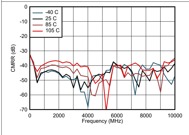
图 6-71. CMRR Across Temperature
