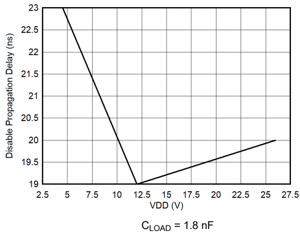
图 6-21. Enable to Output Falling Propagation Delay
