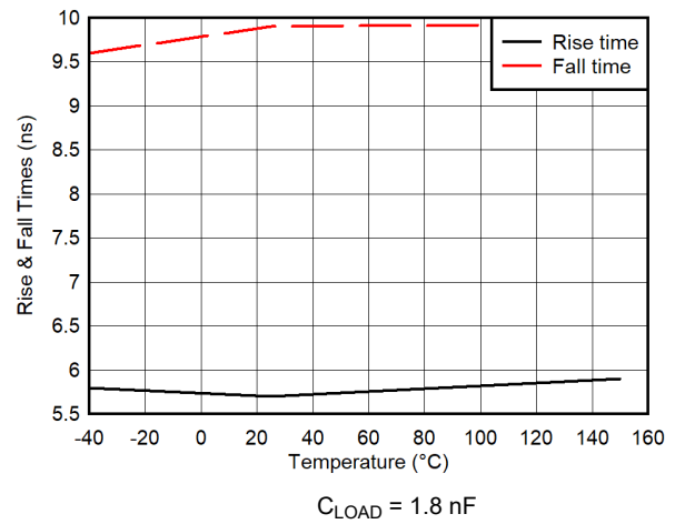
图 6-16. Output Rise and Fall Time vs Temperature
