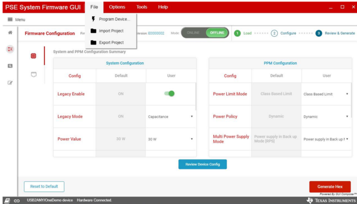
图 9. GUI Program Device and Generate Hex
