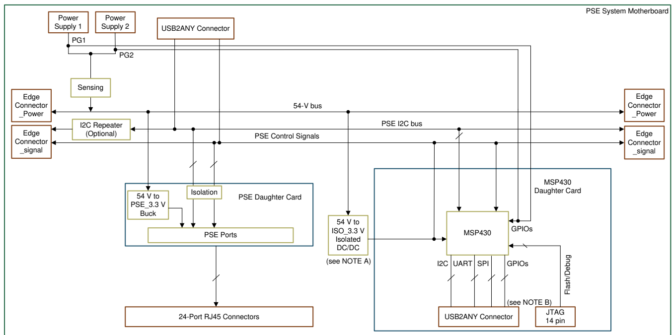
图 1. TIDA-050026-23881 Block Diagram
