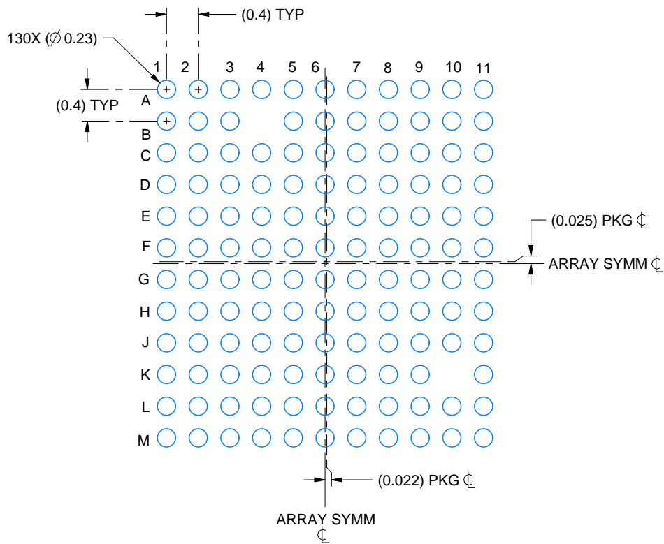
LAND PATTERN EXAMPLE EXPOSED METAL SHOWN SCALE:15X
