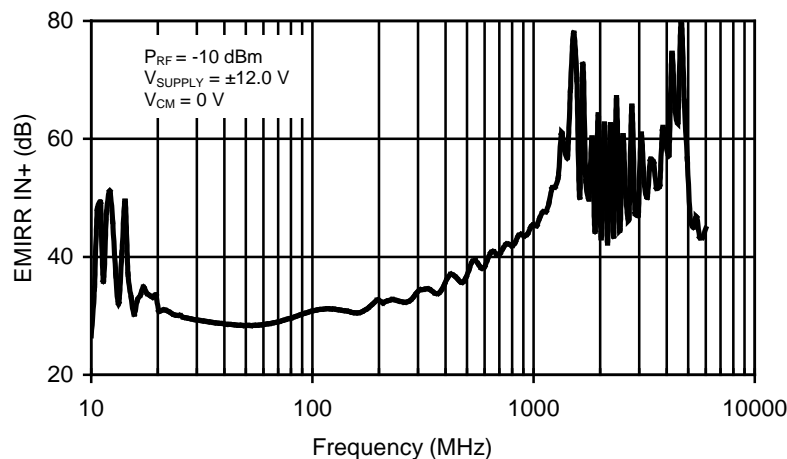
Figure 1. TLE2161 EMIRR IN+ vs Frequency
