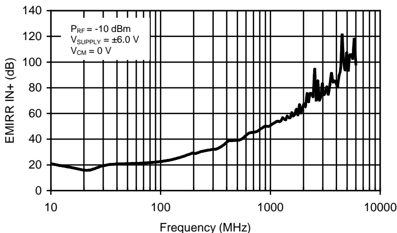
Figure 1. OPA743 EMIRR IN+ vs Frequency
