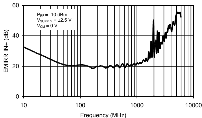
Figure 1. TLV271 EMIRR IN+ vs Frequency
