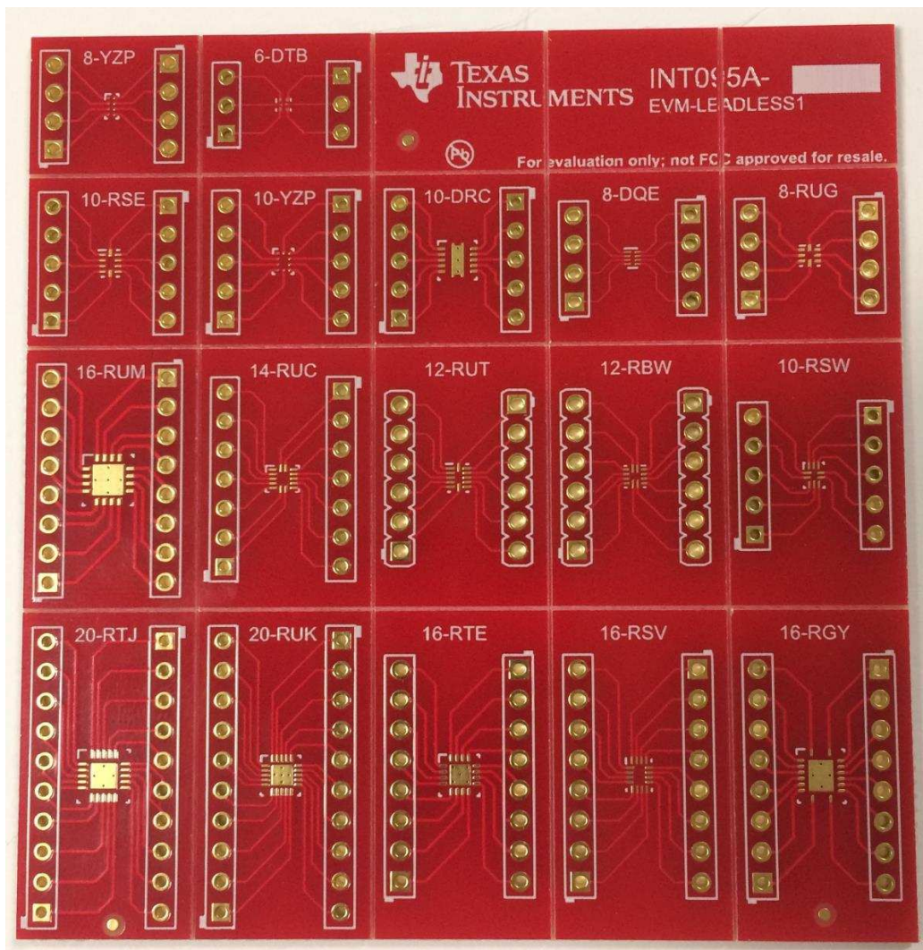
Figure 1. EVM-LEADLESS1-EVM
