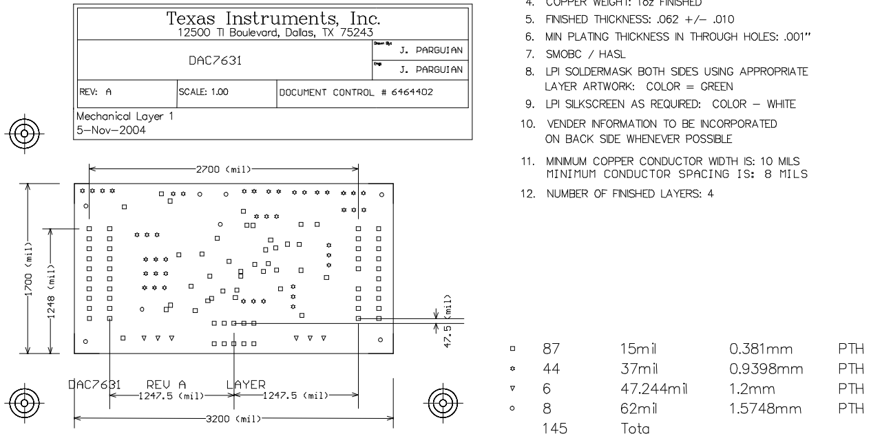
Figure 8. Drill Drawing
