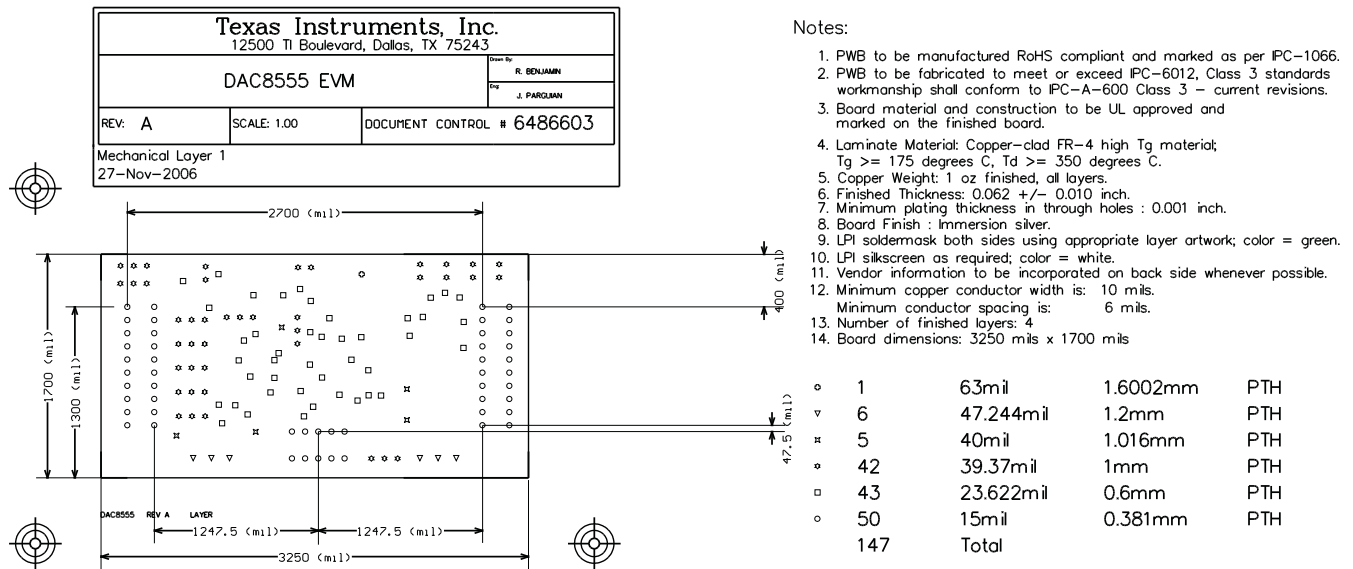
Figure 8. DAC8555EVM—Drill Drawing
