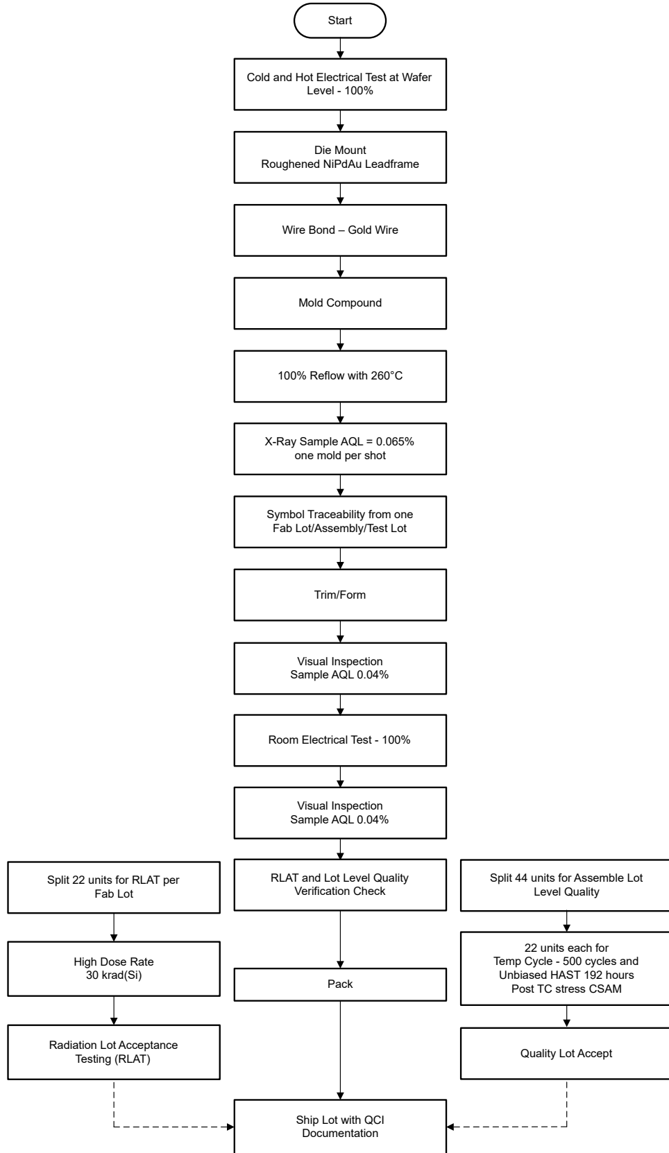
Figure 2-1. LMX1860-SEP Space-Enhanced Plastic Production Flow Chart
